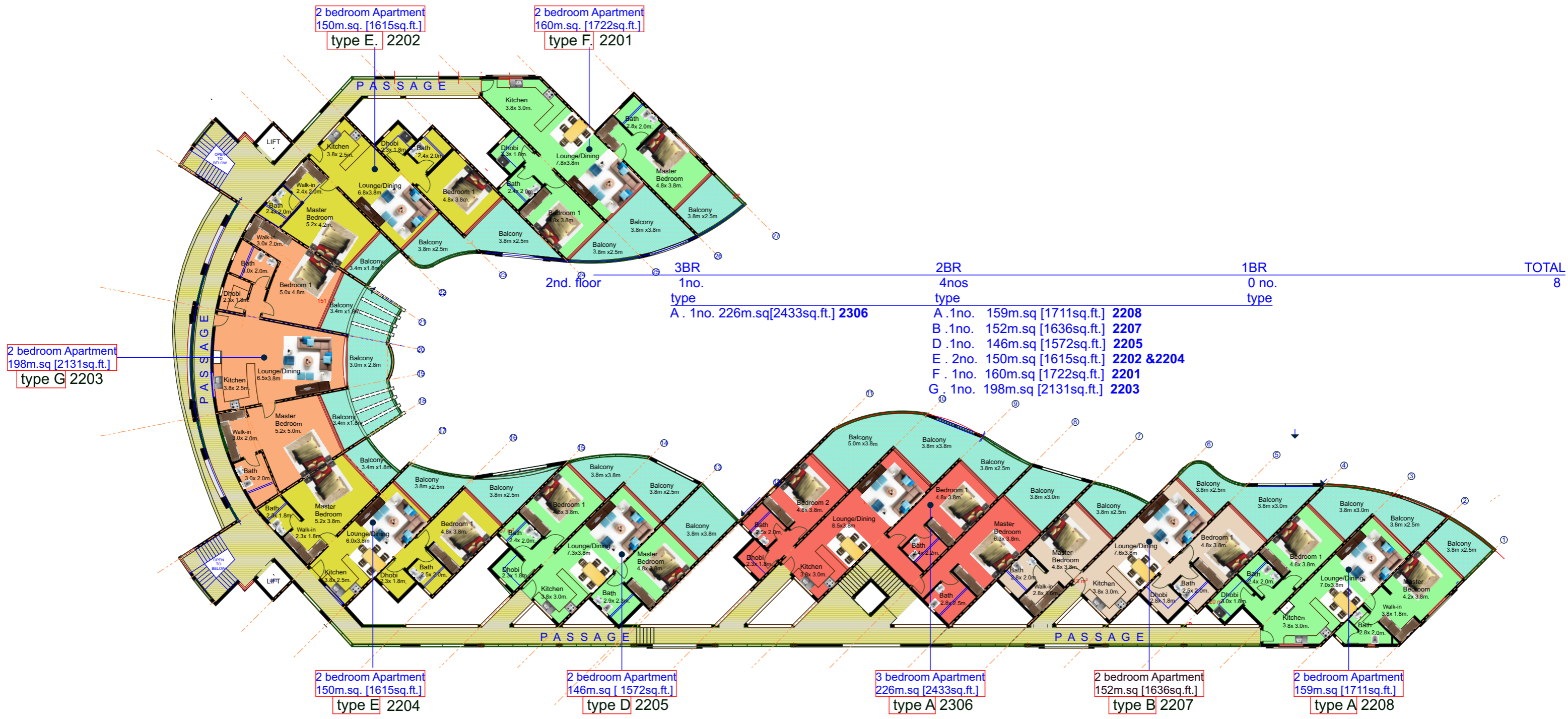
2ND FLOOR PLAN
